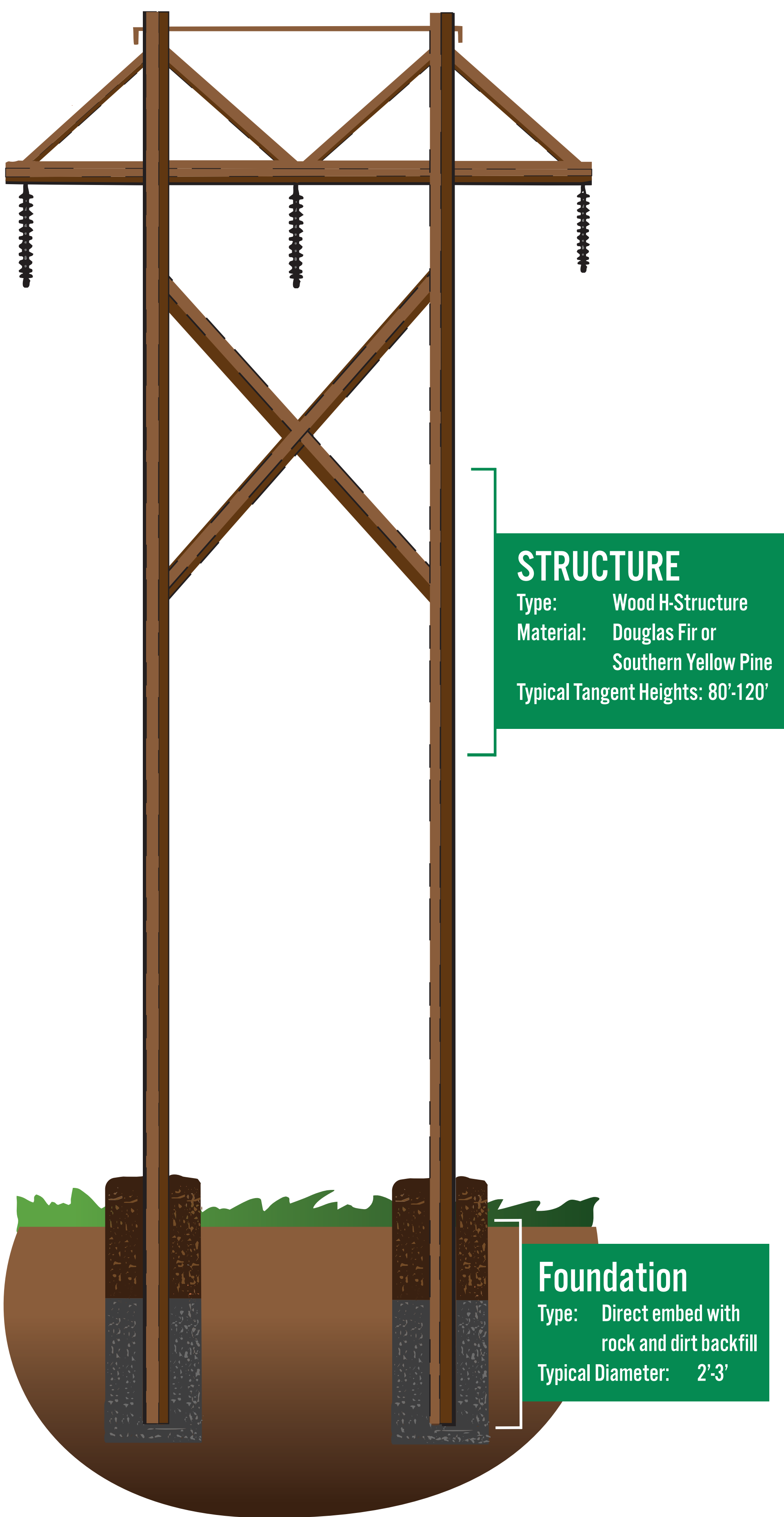
Conceptual H-Structure
