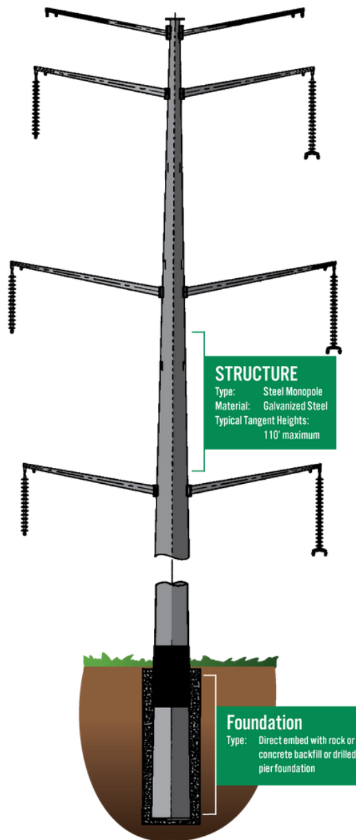
Conceptual Double Circuit Steel Monopole Structure
