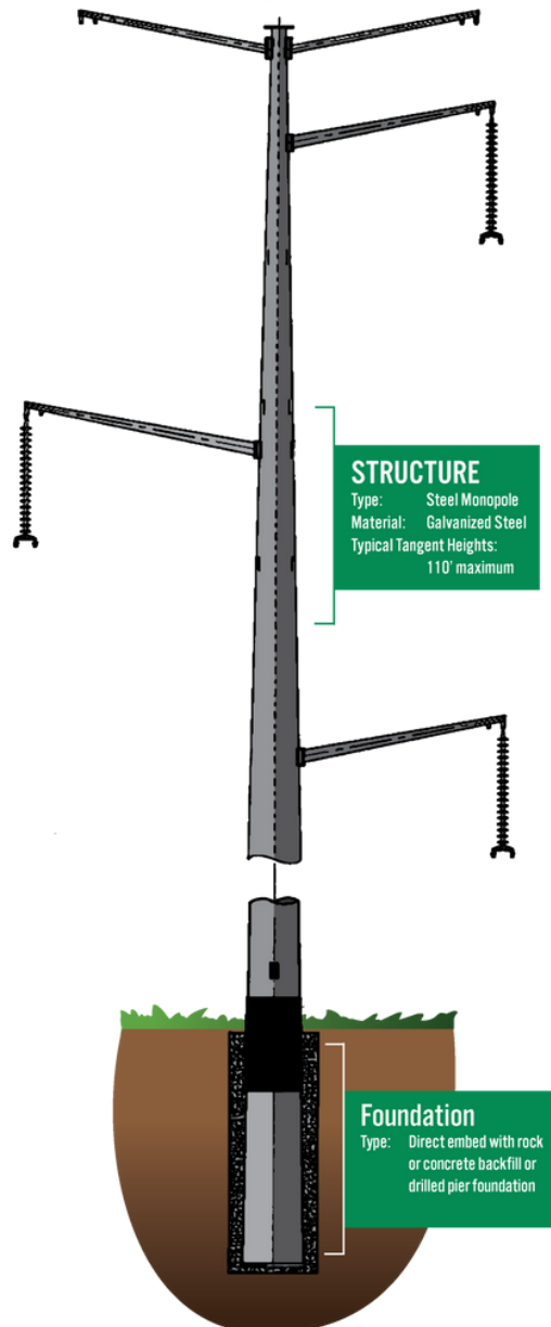
Conceptual Single Circuit Steel Monopole Structure
