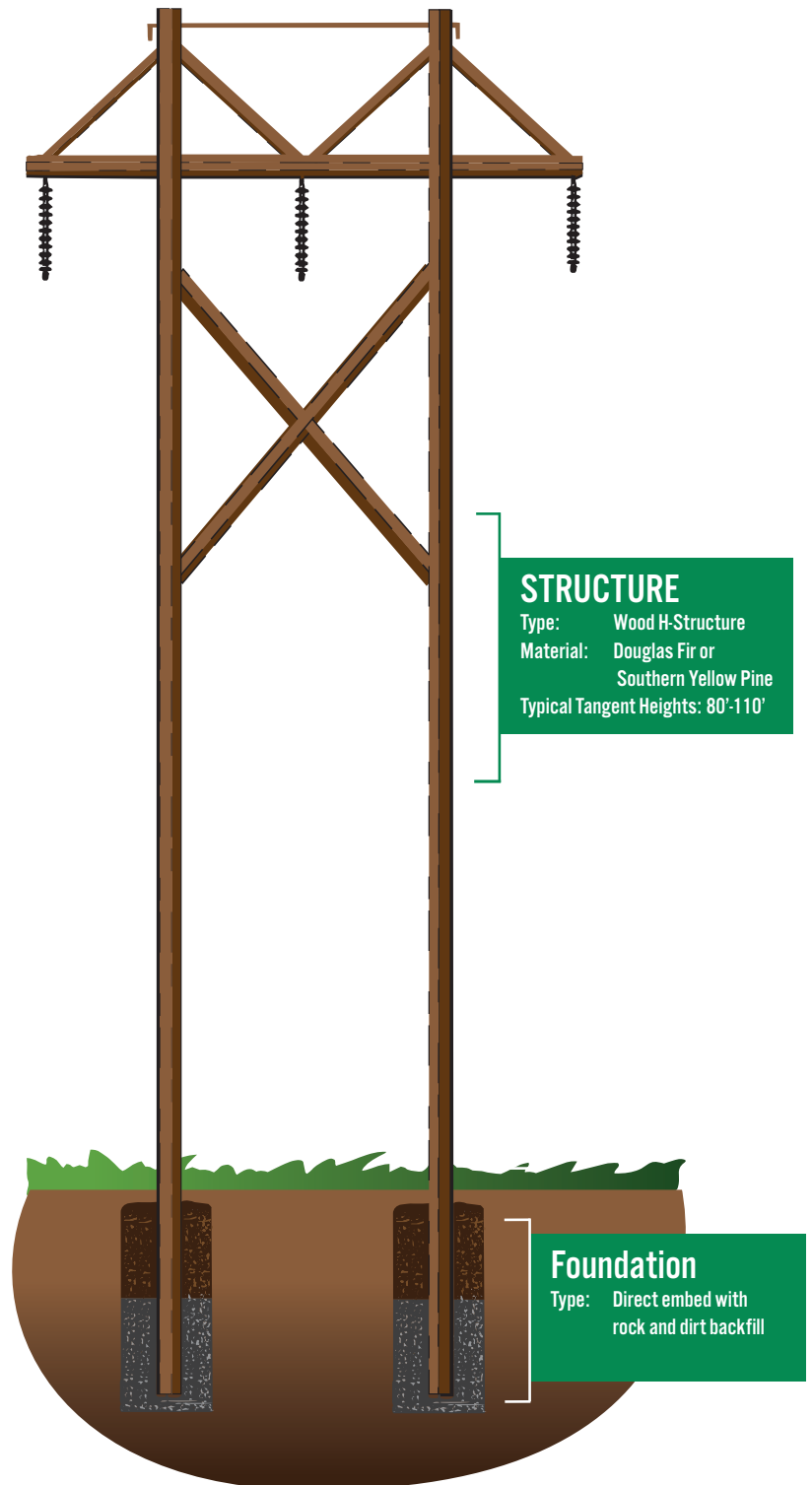
Conceptual Single Circuit Wood H-Structure
