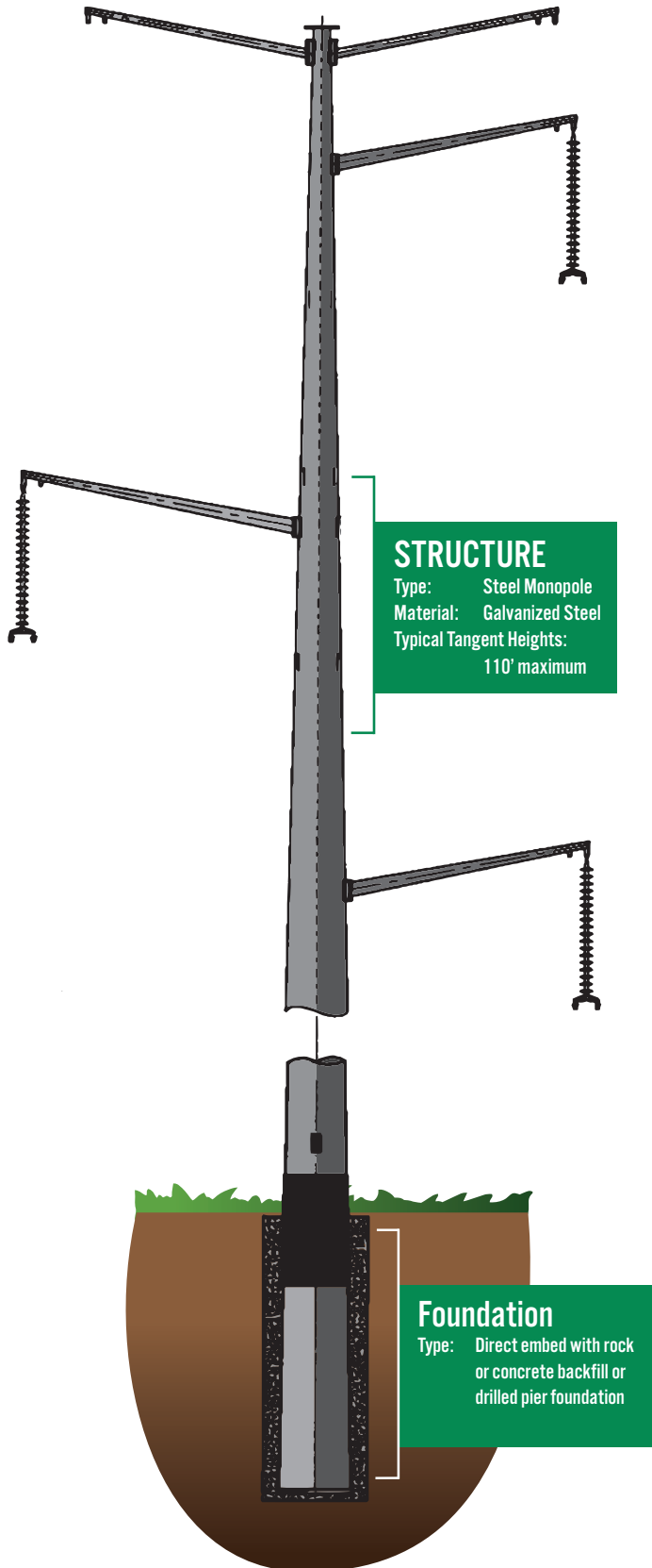
Conceptual Single Circuit Steel Monopole Structure
