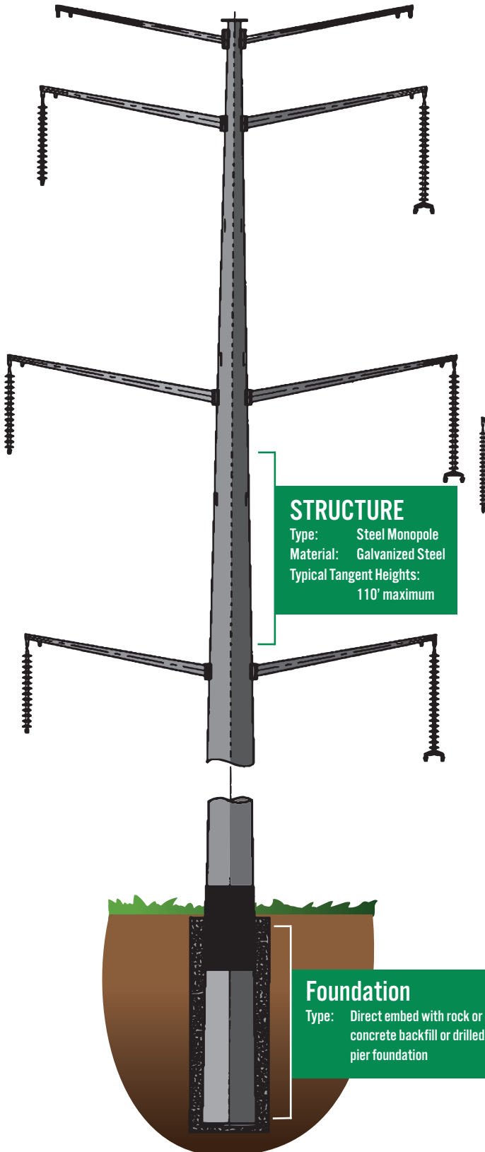
Conceptual Double Circuit Steel Monopole Structure
